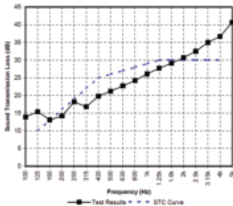
STC 29 - 6kg tested as a free hanging barrier
